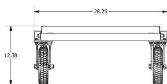
FRONT - STOWED (PANEL REMOVED)
