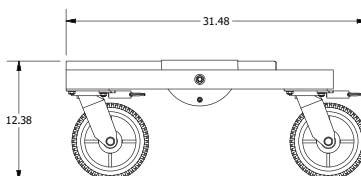
SIDE - STOWED (PANEL REMOVED)
