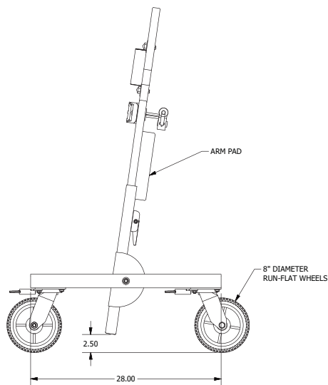
SIDE - DEPLOYED
