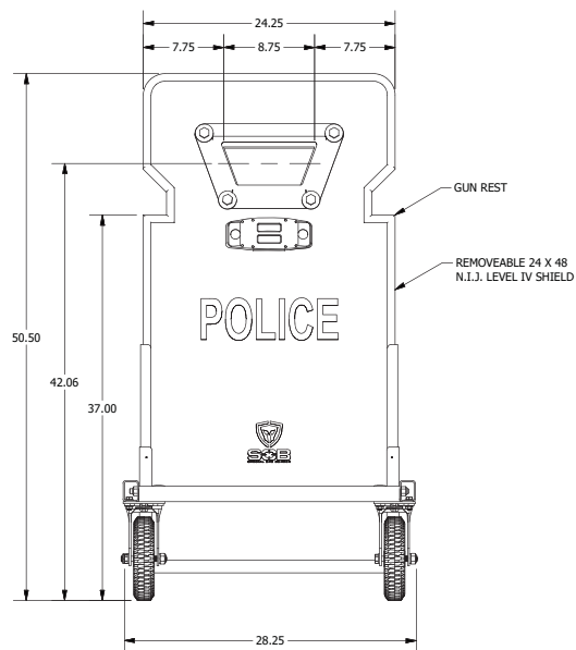
FRONT - DEPLOYED
